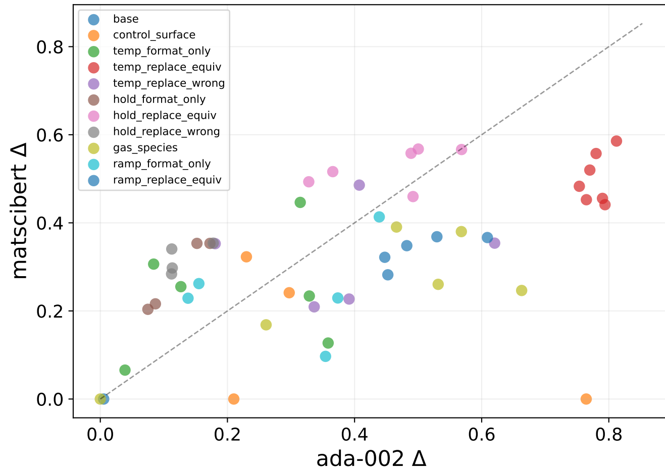
matscibert vs ada-002
